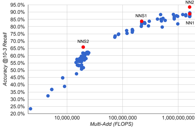
Figure 4. FLOPS vs. Accuracy trade-off. Shown is the trade-off between FLOPS and accuracy for a wide range of different model sizes and architectures. Highlighted are the four models that we focus on in our experiments.
